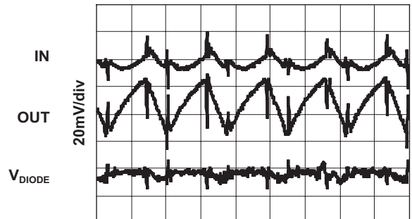
Time (1µs/div)
